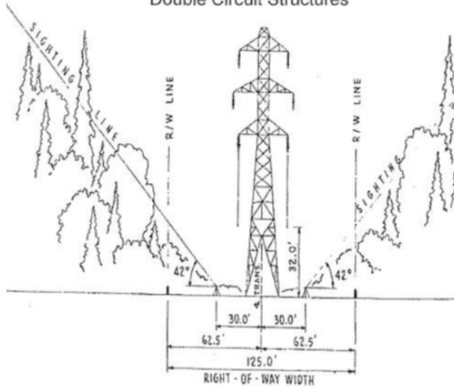
Wire Zone - Border Zone Diagram 230 KV Transmission Line Double Circuit Structures
