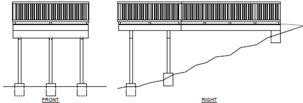
1 PEDESTRIAN BRIDGE ELEVATIONS D1.0 1/4" = 1'-0"
